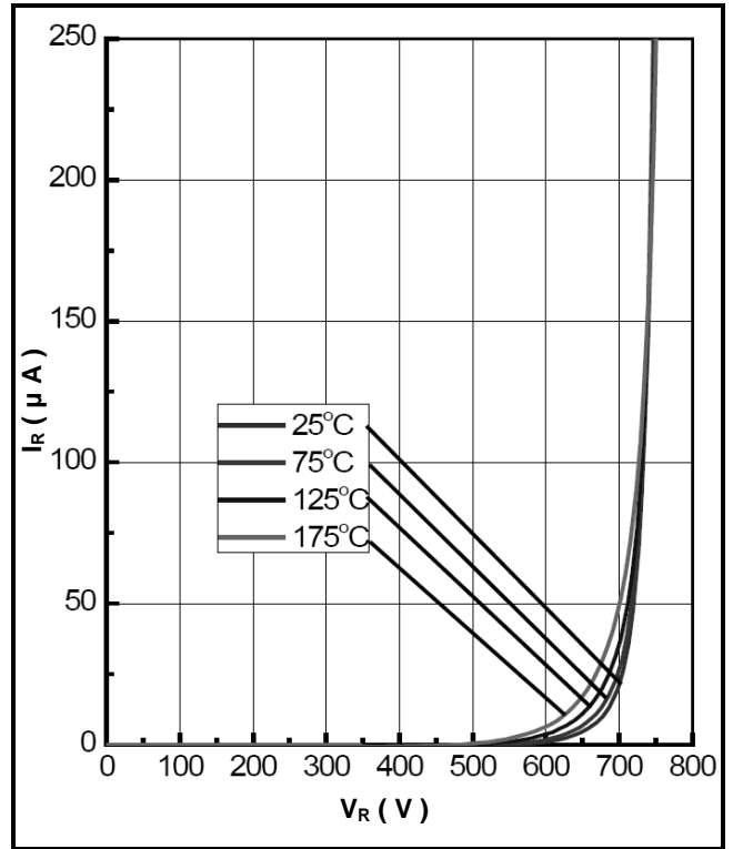
Figure 2. Reverse Characteristics
