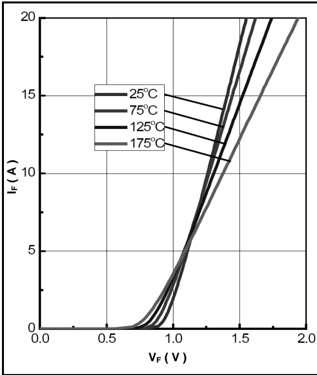
Figure 1. Forward Characteristics
